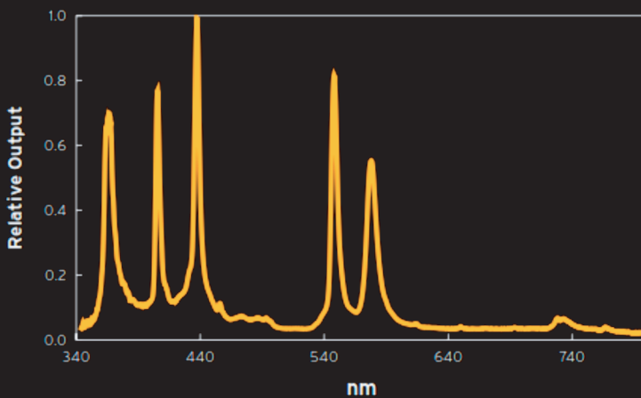
Wide output spectrum similar to Hg
